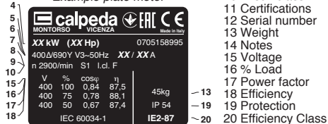
Example plate motor
